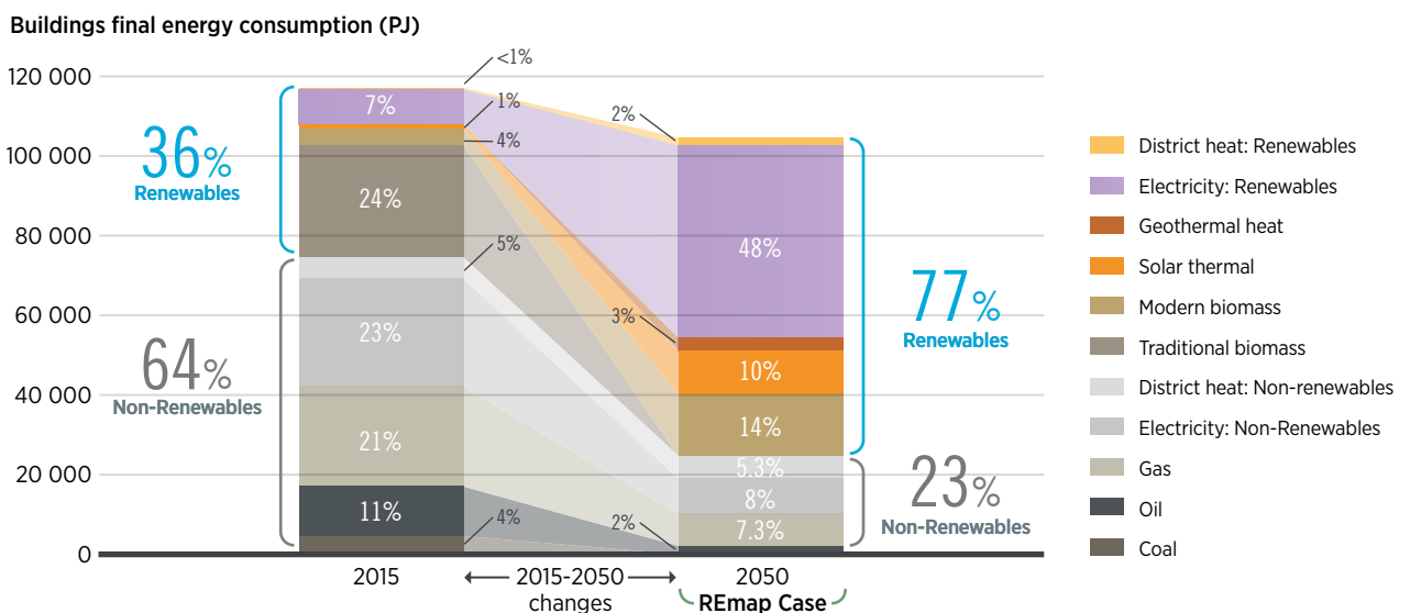
Figure 12. The increasing use of electricity in buildings and the decline of fossil fuels Breakdown of final energy consumption in the building sector, by source (PJ/yr)
